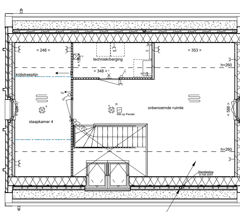
zolder
