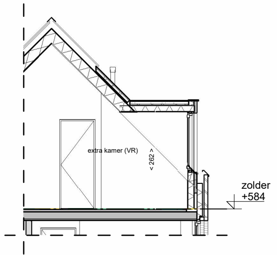
code 10600: dakkapel
